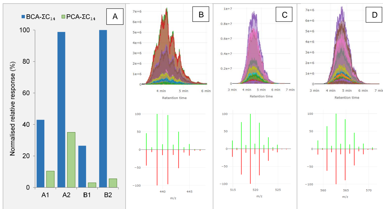
Figure 1. A: Normalised relative response (%) of \Sigma\text{BCA-C}_{14} and \Sigma\text{PCA-C}_{14} detected as [\text{M} + \text{Cl}]^- in synthesized standards. B, C and D: Example chromatograms and mass spectra of [\text{M} + \text{Cl}]^- for \text{C}_{14}\text{H}_{24}\text{Cl}_6 , \text{C}_{14}\text{H}_{23}\text{BrCl}_6 and \text{C}_{14}\text{H}_{23}\text{Br}_2\text{Cl}_5 isotopomers, respectively, in synthesised standard A2, generated by CP-Seeker software. Chromatograms display overlaid results for each of the detected isotopomers. Mass spectra show measured profile above (green) and theoretical profile below (red). Mass spectra in Figures B, C, and D had isotopic pattern match scores of 98, 97 and 95%, respectively, and mass deviation of 0.58, 0.55 and 0.50 mDa, respectively, compared with theoretical values.
