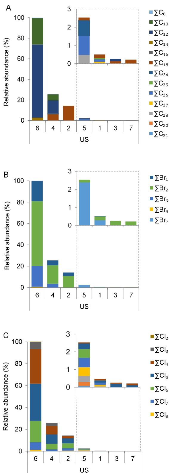
Figure 3. Normalised relative response (%) of BCA homologue groups detected in indoor dust samples grouped by A) carbon, B) bromine and C) chlorine numbers.
