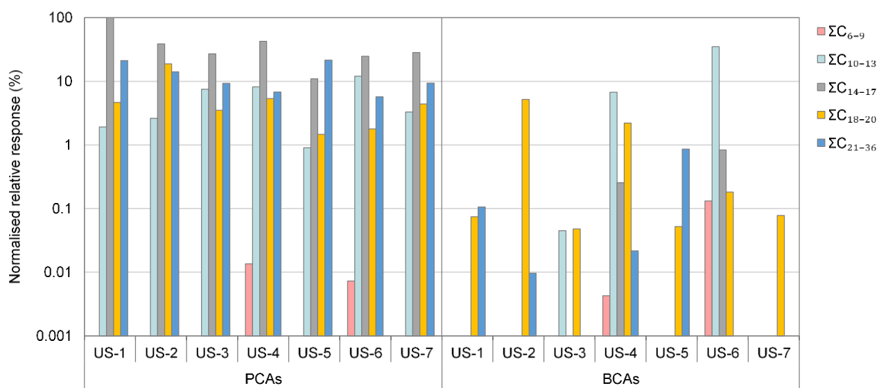
Figure 5. Normalised relative response (%) of PCAs and BCAs grouped by carbon chain length.
