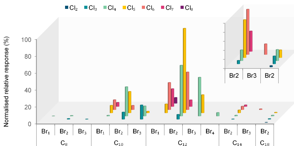
Figure 4. Normalised relative response of BCA homologue groups detected in indoor dust sample US-6.
