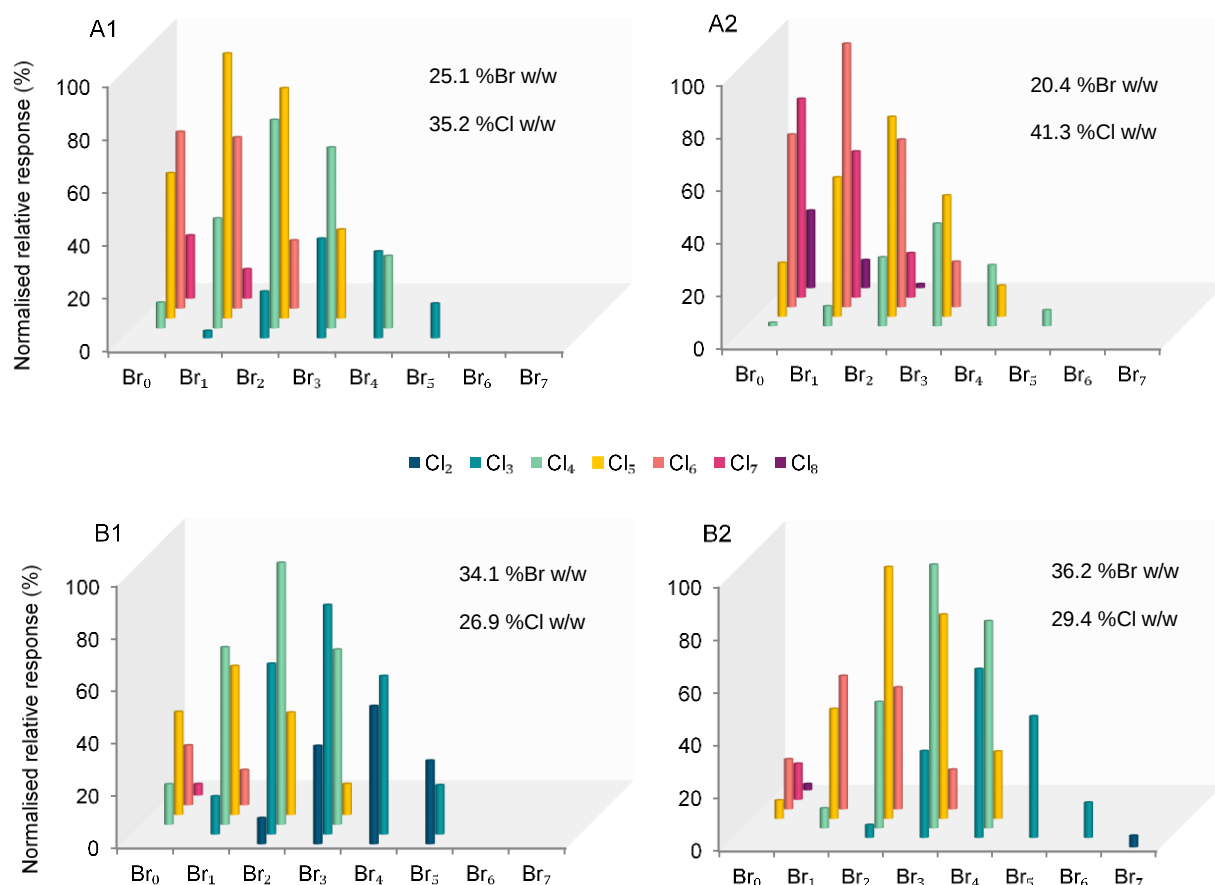
Figure 2. Normalised relative response (%) of bromine and chlorine on \text{C}_{14} n -alkane chains of synthesised standards A1, A2, B1 and B2, normalised per individual standard. Br and Cl mass fractions (% w/w) indicated on Figures account for BCA and PCA ( \text{Br}_0 ) homologue groups detected by LC-ESI-Orbitrap analysis.
